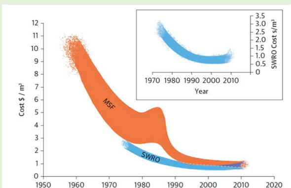
Desalination costs (Sources: World Bank. 2019. "The Role of Desalination in an Increasingly Water-Scarce World." World Bank, Washington, DC. | Elimelech and Philip)
