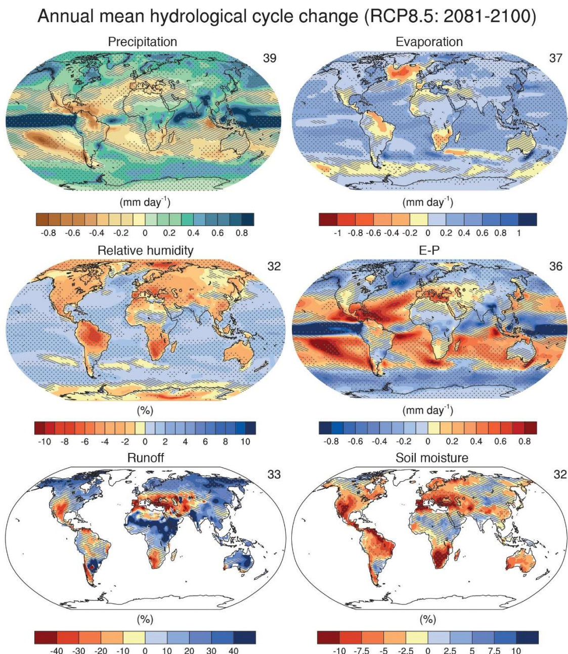
Figure 3-7: Annual mean changes in precipitation (P), evaporation (E), relative humidity, E – P, runoff and soil moisture for 2081–2100 relative to 1986–2005 under the Representative Concentration Pathway RCP8.5. Illustration from IPCC report, 2013 (Stocker, et al., 2013).
