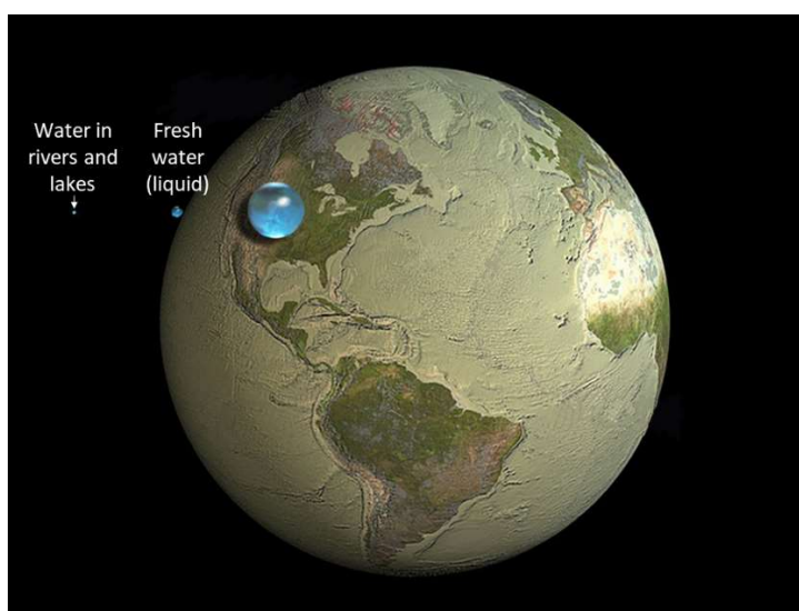
Figure 3-1: The blue spheres represent the relative amounts of terrestrial water compared to Earth's size. The largest sphere's volume represents the total amount of water in, on, and above the Earth (1,385 km in diameter). The freshwater (liquid) sphere represents groundwater, swamps, rivers, and lakes (272.8 km in diameter). The smaller sphere represents water from rivers and lakes (56.2 km in diameter). Image-based on an illustration from the U. S. Geological Survey (Perlman, Cook, Hole, Woods, & Nieman., 2016).
